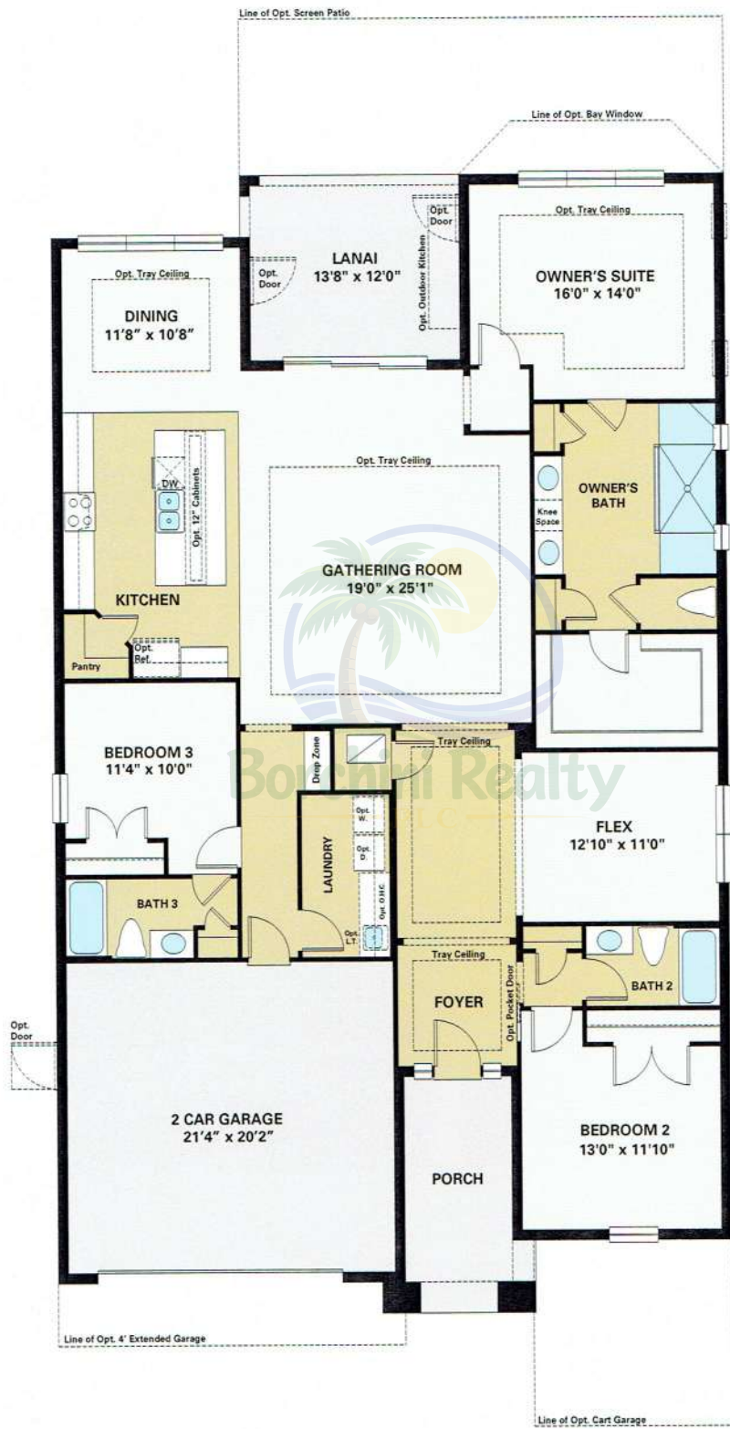
FLOOR PLAN
